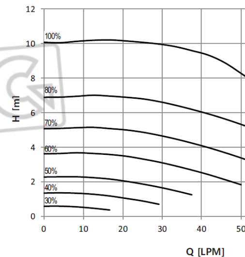
Q-H Chart
