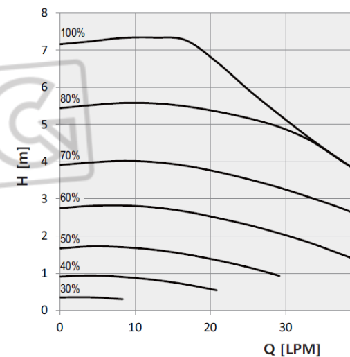
Q-H Chart
